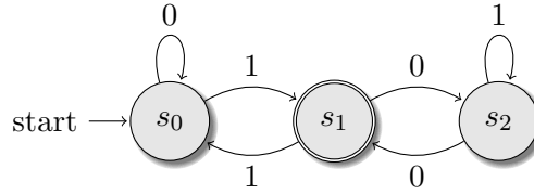
Figure 1: A 3-state Deterministic Finite Automata M .
